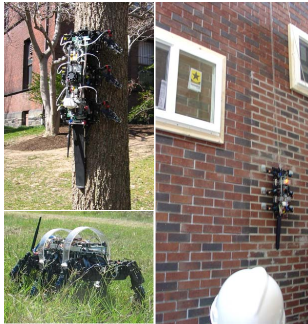
Figure 7: The RiSE platform is capable of scaling a wide variety of real world surface types and variations as well as maintaining capable level ground locomotion. Clockwise from the upper left, RiSE is climbing a tree, climbing a brick wall, and walking through tall grass.
