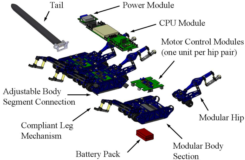
Figure 2: RiSE’s modular design allows for easy reconfiguration of the different leg segments. Each module contains four motors, a four axis motor amplifier, and one battery pack.
