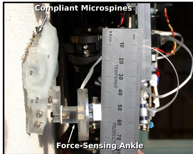
Figure 6. Photo of a RiSE foot and ankle engaged on a stucco surface. Each microspine is individually compliant, to catch onto surface asperities. A force sensing device measures the forces felt at the ankle.
